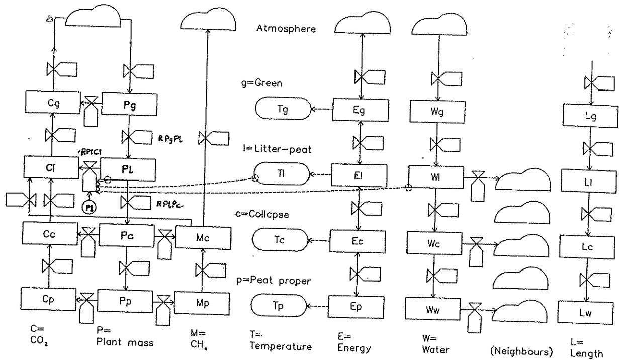
Fig. 7. Outline of a Forrester simulation model of an element of a peatland. It includes flows of \text{CO}_2 (C), plant/peat organic matter (P), \text{CH}_4 (M), energy (E), water (W), 'length' (L), and the derived property temperature (T). The four layers correspond to those in Fig. 2: green (g), litter-peat (l), collapse (c) and peat proper (p). In practice it might be useful to subdivide some of these. In order to run the model the functional relations of all the valves would need to be known or assumed. Only one is shown — that from PI to CI. The rate \text{RPICl} is shown as determined by the difference equation version of equation (3) and, in an unspecified way by temperature and water content.
