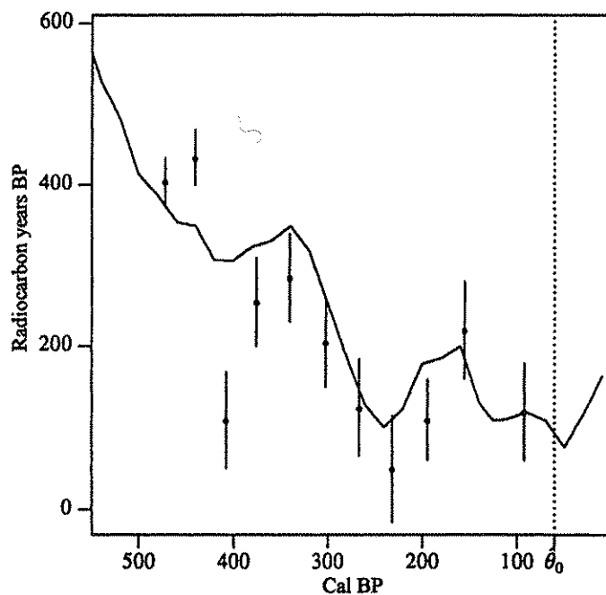
Fig. 4 ^{14}\text{C} dates from the peat core from Ellergower Moss with the relevant part of the calibration curve. \bullet = ^{14}\text{C} age x_i ; — = x_i - \sigma_i to x_i + \sigma_i . Here we used the modal values of the joint posterior distribution of \theta_0 and p , taking \theta_0 = 61 yr and p = 0.0054 \text{ g cm}^{-2} \text{ yr}^{-1} .
